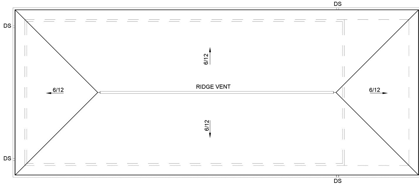
1 GARAGE TYPE 1 ROOF PLAN A4.11 SCALE 1/4"=1'
