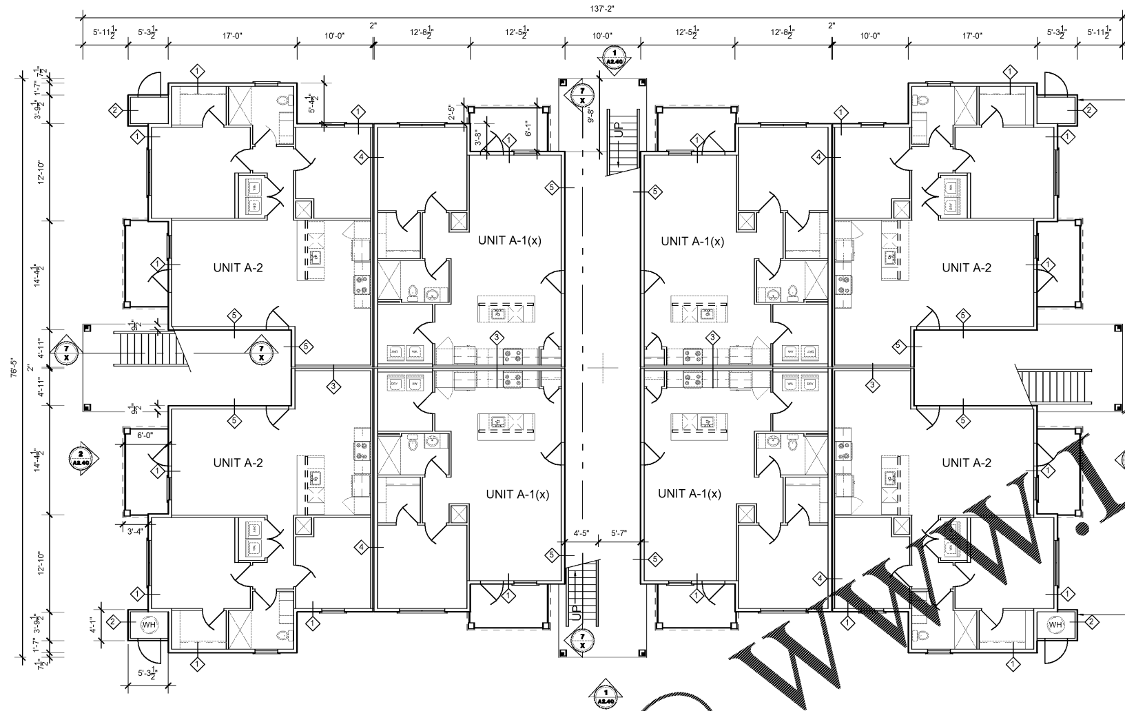
1 BLDG TYPE 4 (BUILDINGS 3, & 6): FIRST FLOOR PLAN A1.41 SCALE 1/8"=1'
