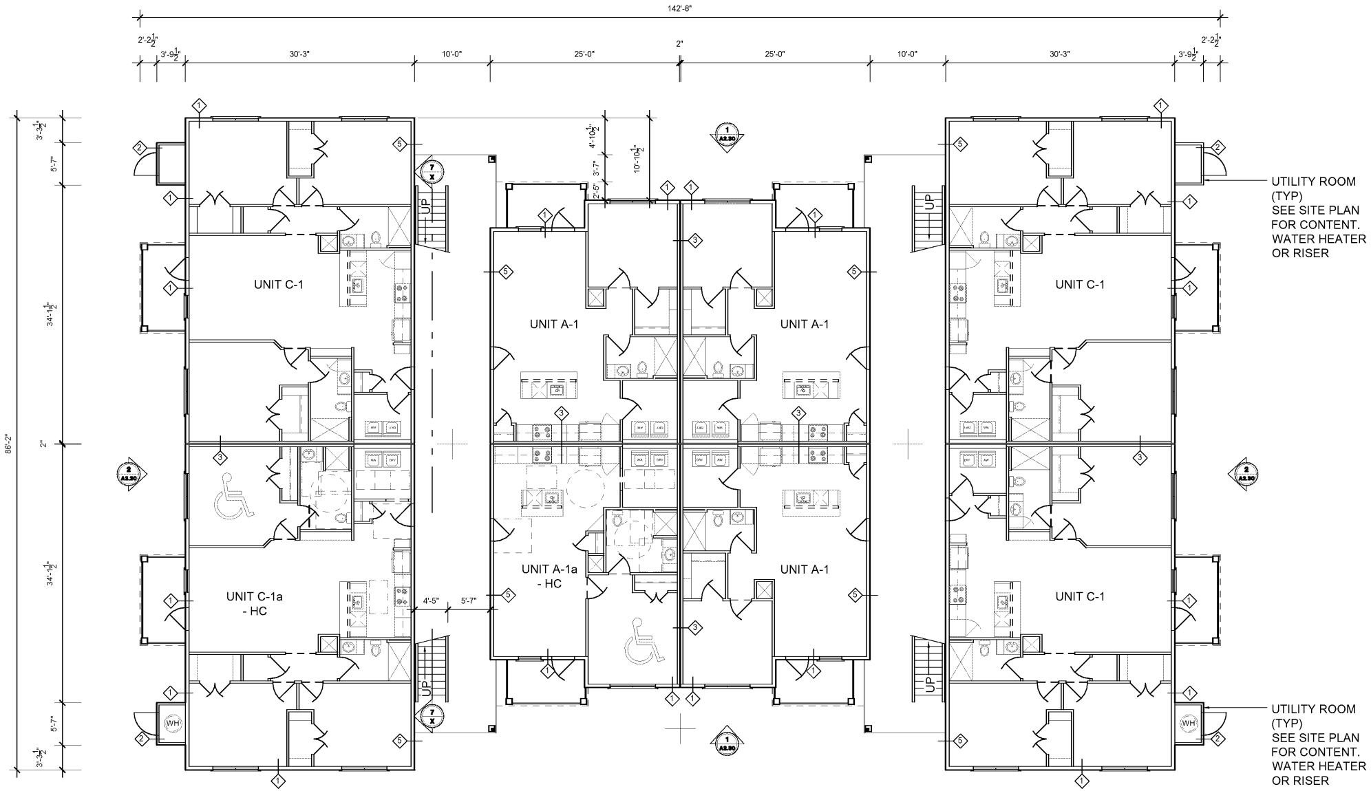
1 A1.31b BLDG TYPE 3b (BUILDING 7) FIRST FLOOR SCALE 1/8"=1'
