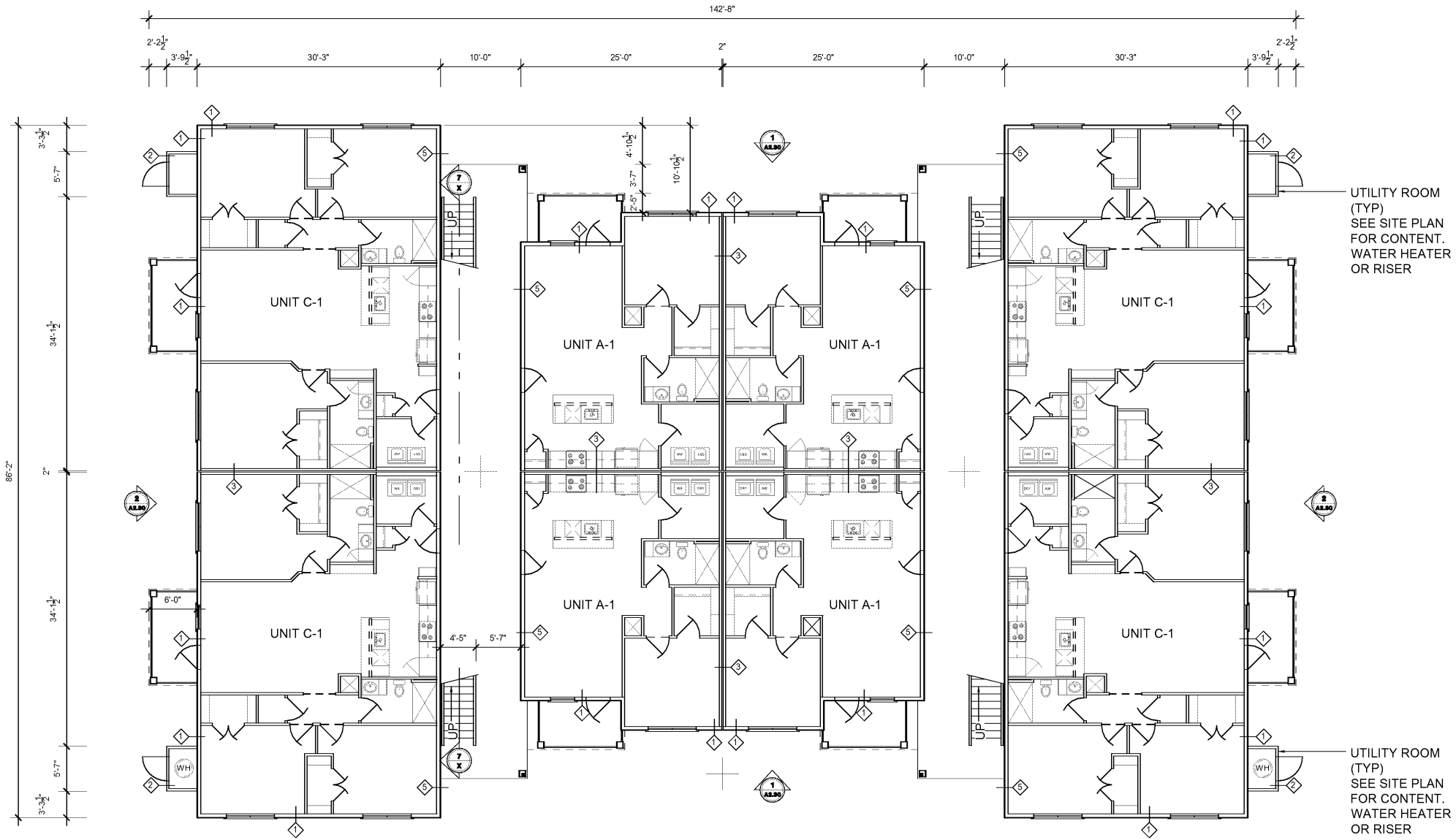
1 BLDG TYPE 3 (BUILDING 2): FIRST FLOOR A1.31 SCALE 1/8"=1'
