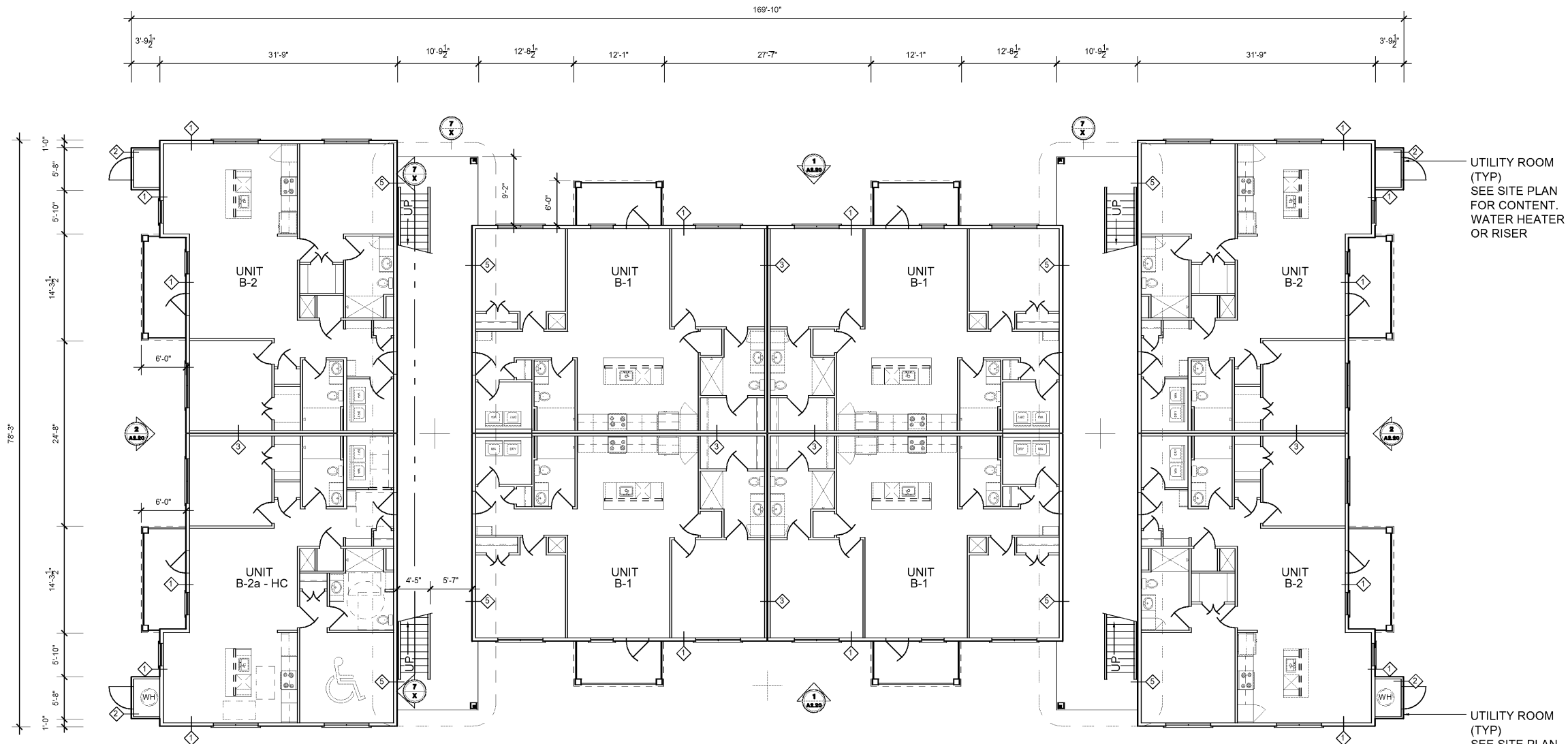
1 BLDG TYPE 2A (BUILDINGS 1,8,&12 ): FIRST FLOOR A1.21a SCALE 1/8"=1'
