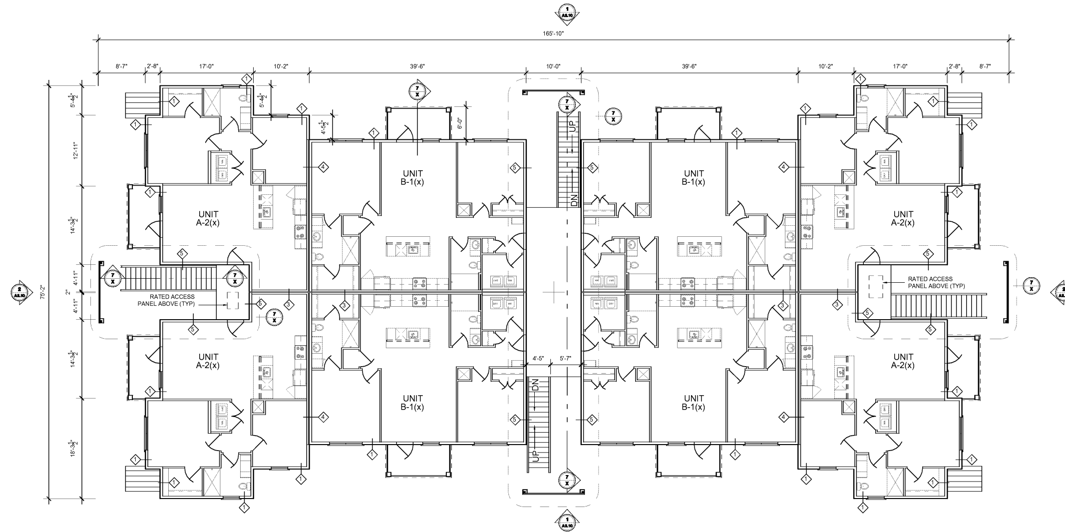
1 BLDG TYPE 1 (BUILDINGS 9,10,11,&14): SECOND FLOOR PLAN A1.12 SCALE 1/8"=1'
