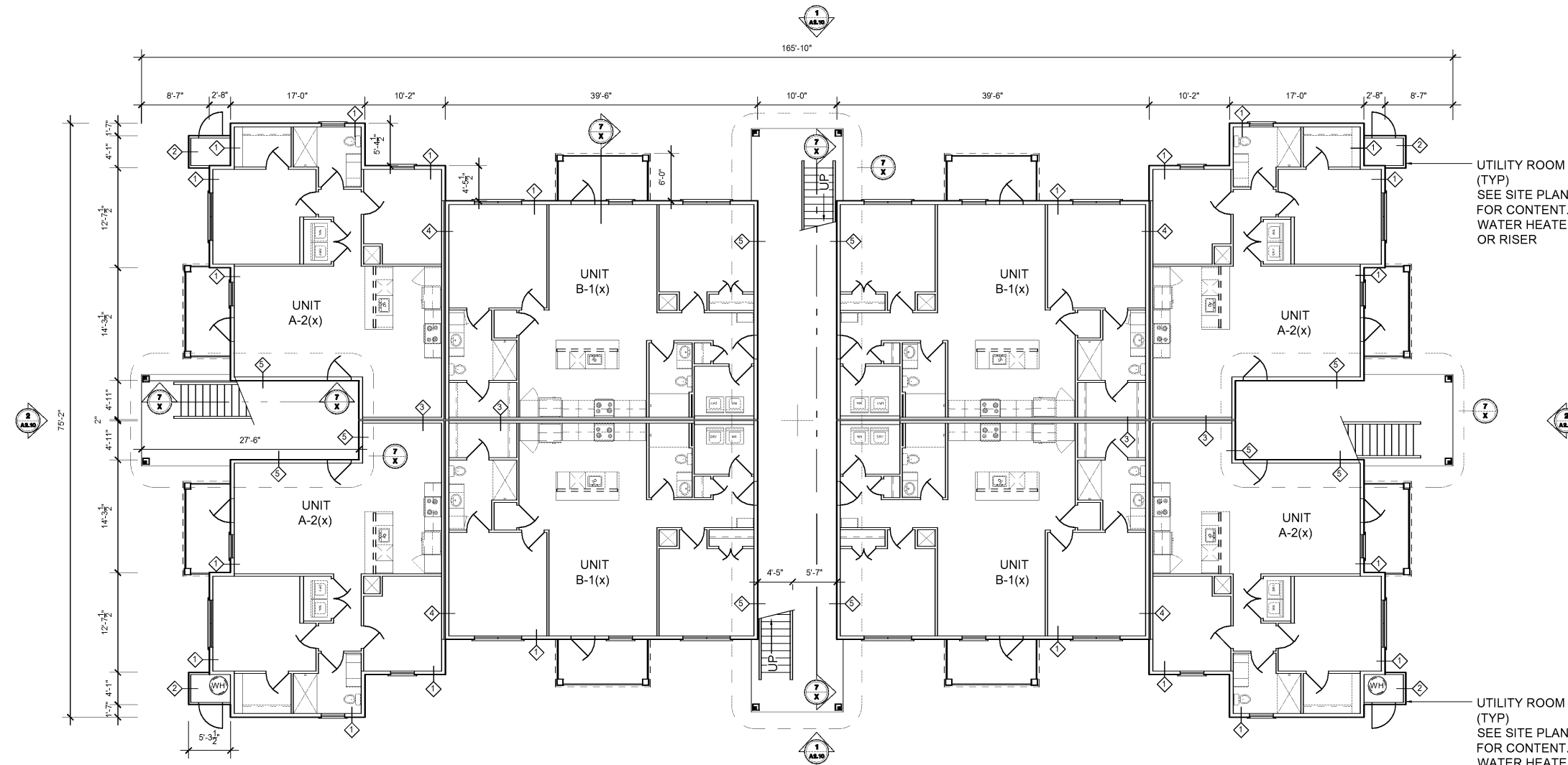
1 BLDG TYPE 1 (BUILDINGS 9,10,11,&14): FIRST FLOOR PLAN A1.11 SCALE 1/8"=1'
