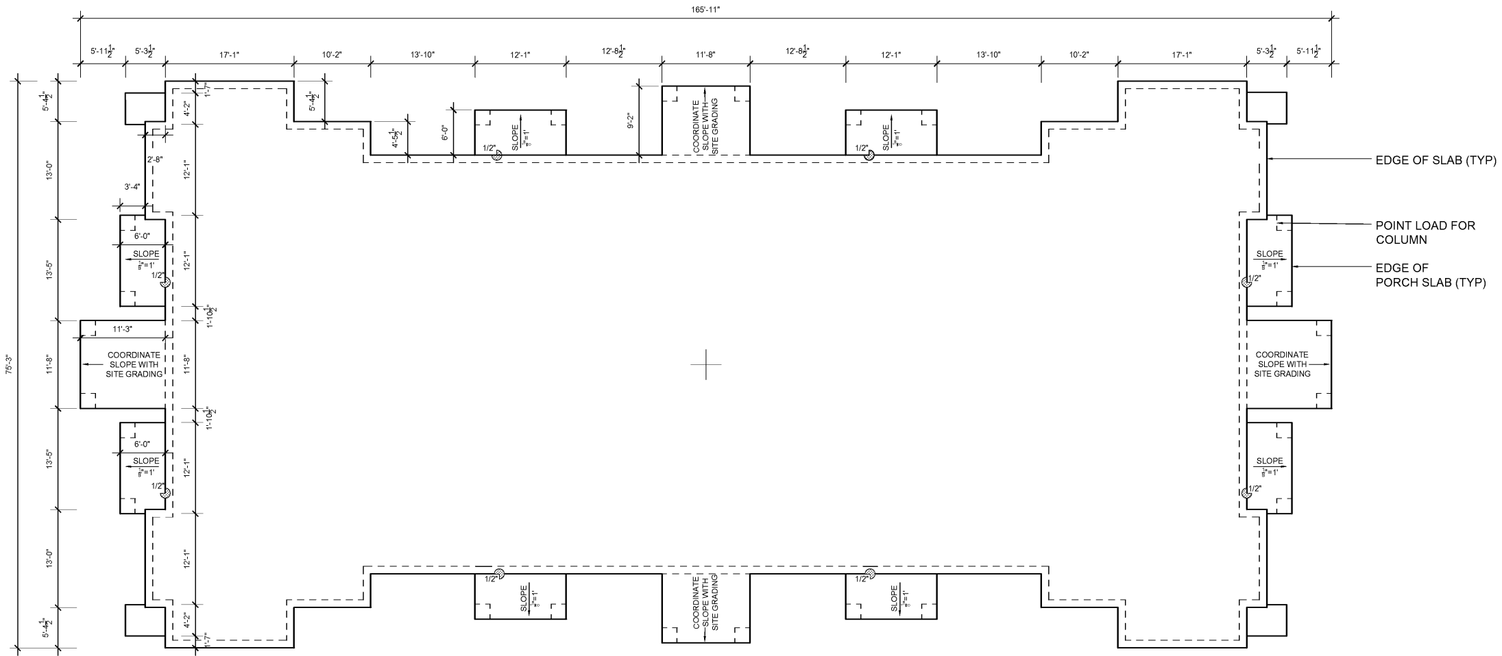
1 BLDG TYPE 1 (BUILDINGS 9,10,11,&14): EDGE OF SLAB PLAN A1.10 SCALE 1/8"=1'
