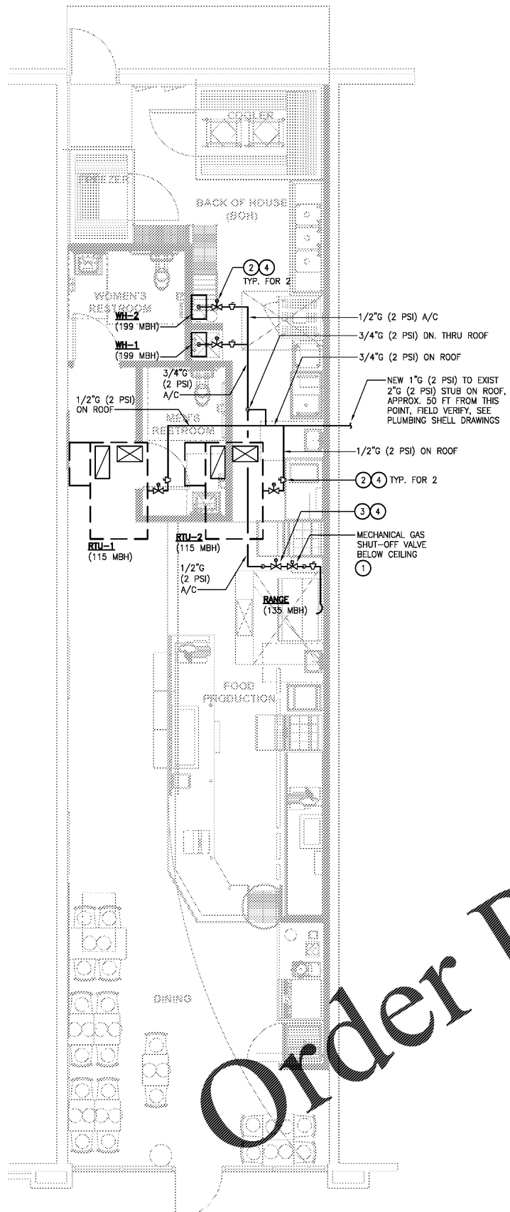
1 GAS SUPPLY FLOOR PLAN P1.01 SCALE: 1/4" = 1'-0"
