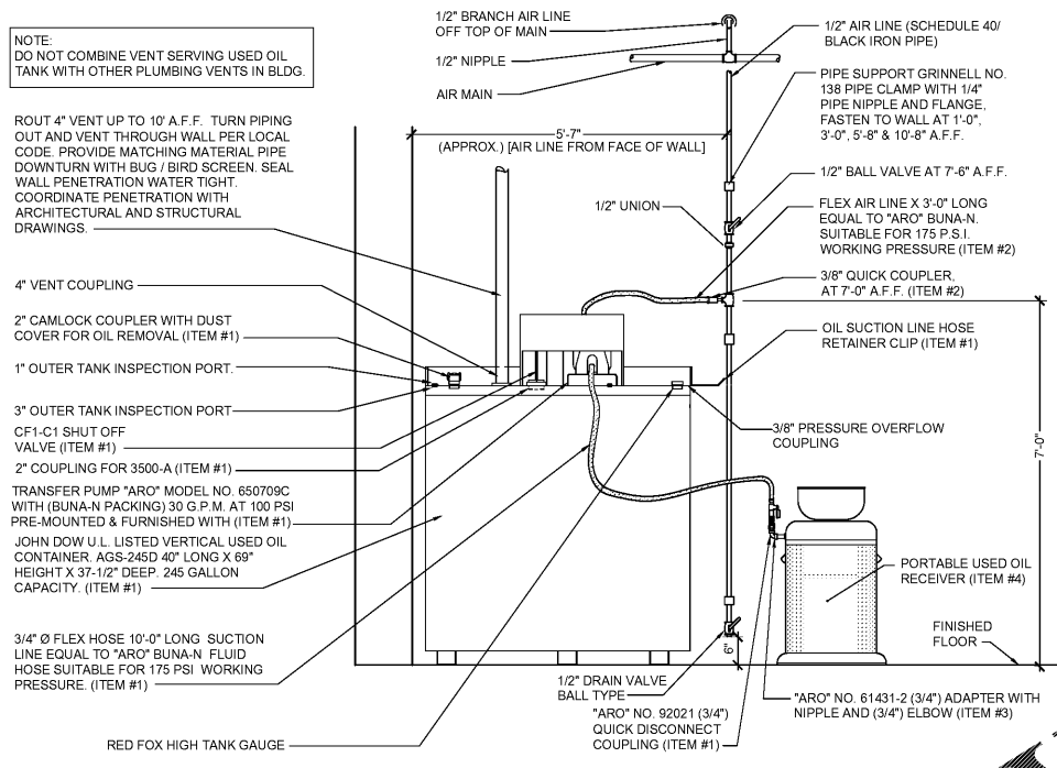
1 USED OIL STORAGE SYSTEM ELEVATION VIEW P4 SCALE: N.T.S.
