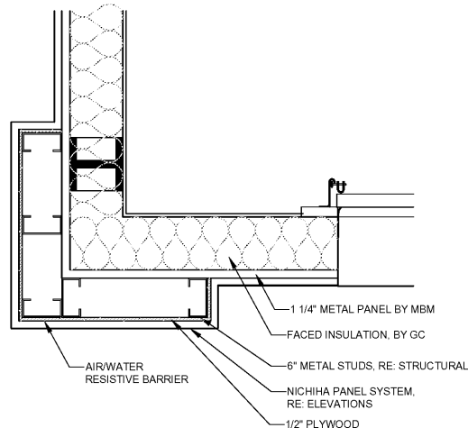
1 ENLARGED PLAN DETAIL A1.2 SCALE: 1"=1'-0"
