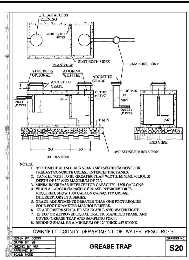
GREASE TRAP DRAWING NO. S20
