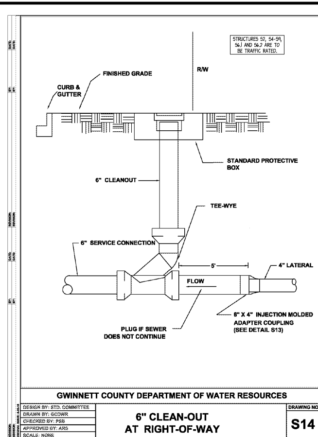
6" CLEAN-OUT AT RIGHT-OF-WAY DRAWING NO. S14
