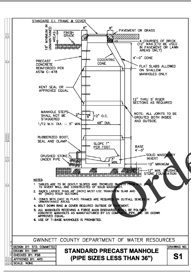
STANDARD PRECAST MANHOLE (PIPE SIZES LESS THAN 36") DRAWING NO. S1
