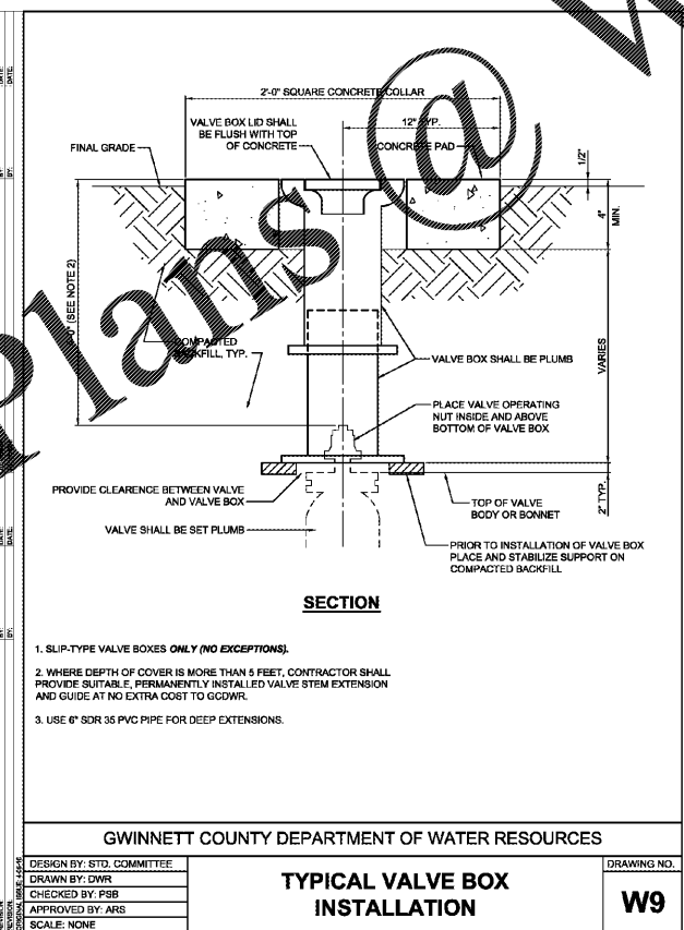
6 VALVE BOX INSTALLATION NTS
