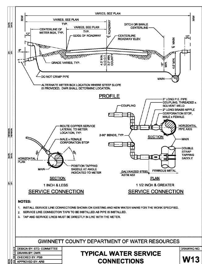
8 WATER SERVICE CONNECTIONS NTS
