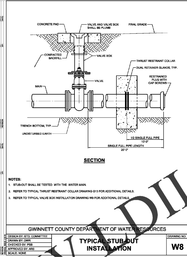
3 STUB-OUT INSTALLATION NTS
