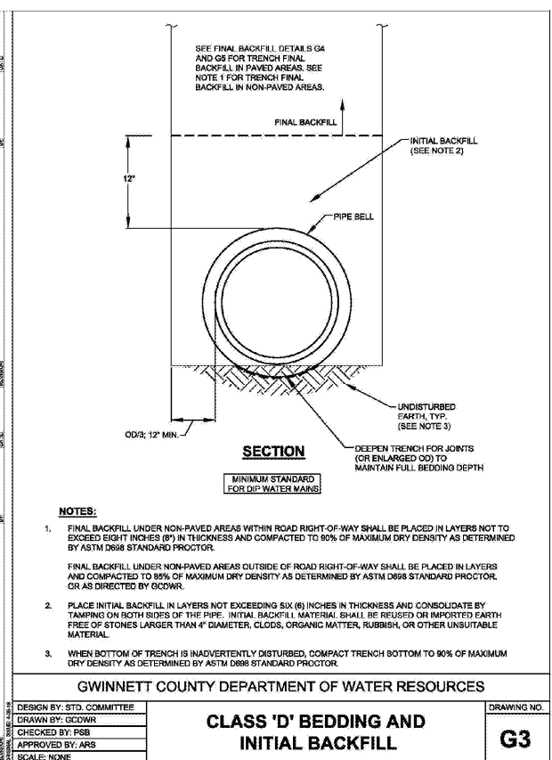
7 WATER BEDDING & BACKFILL NTS
