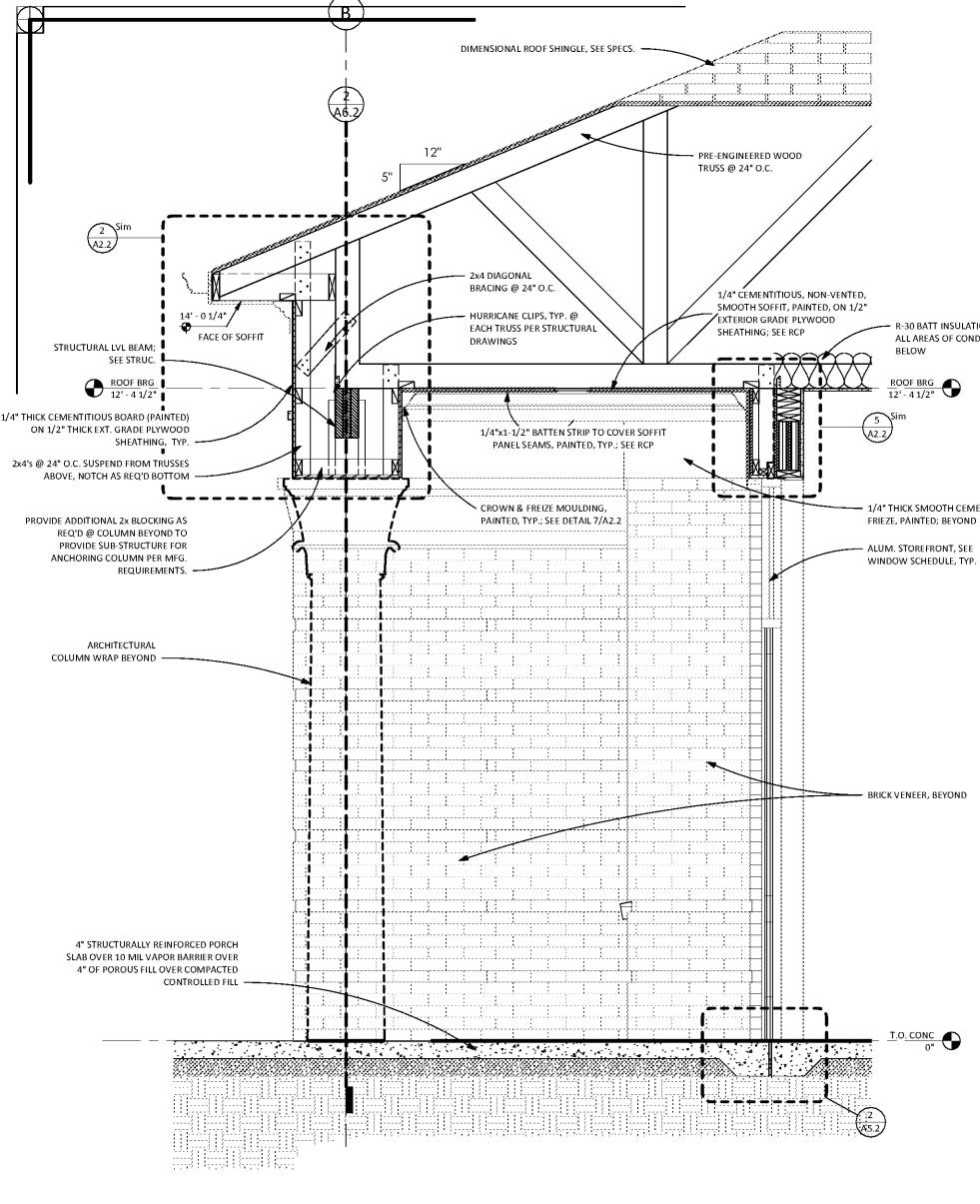
1 WALL SECTION @ ENTRY PORTICO A7.1 3/4" = 1'-0"
