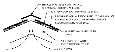
3 SHINGLE OVER RIDGE VENT DETAIL A3.1 1 1/2" = 1'-0"
