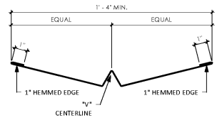
4 TYP. VALLEY FLASHING DETAIL A3.1 3" = 1'-0"
