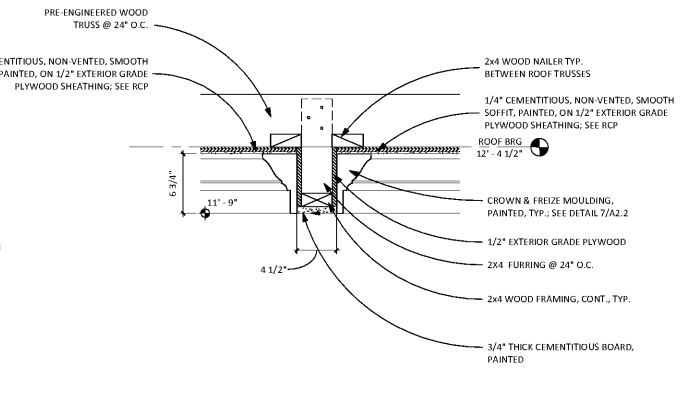
4 PORCH SOFFIT/COFFER DETAIL 1 1/2" = 1'-0"
