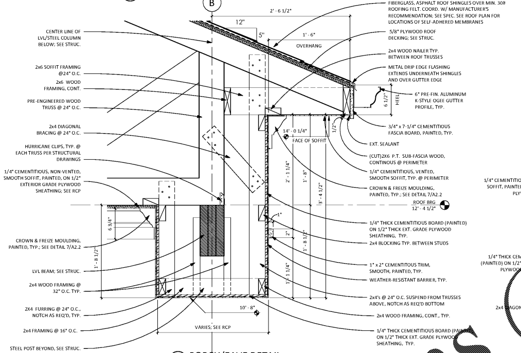
2 PORCH/EAVE DETAIL 1 1/2" = 1'-0"
