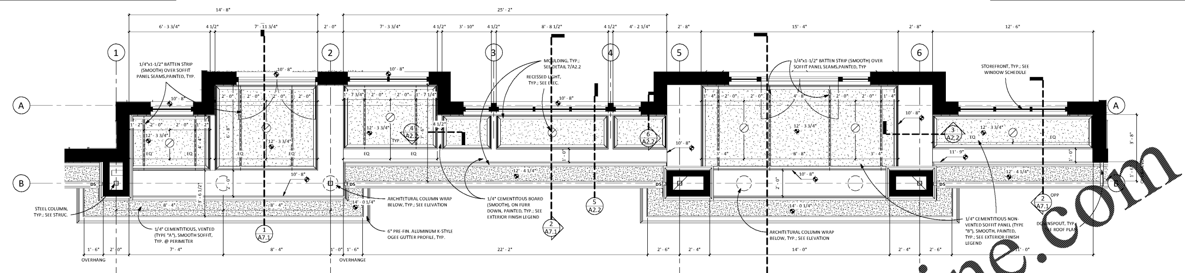
1 ENLARGED RCP - FRONT PORCH 3/8" = 1'-0"
