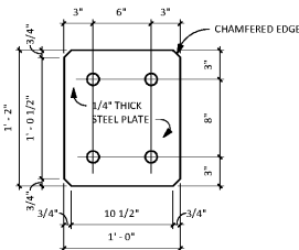
3 CANE BOLT BASE PLATE A0.3 1 1/2" = 1'-0"
