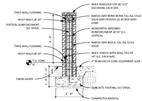
8 TYPICAL MASONRY MECHANICAL SCREEN WALL A0.3 1/2" = 1'-0"
