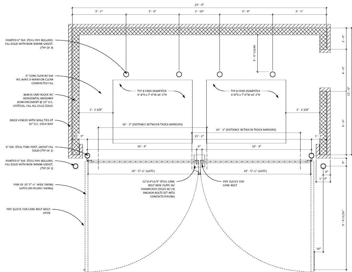
1 DOUBLE DUMPSTER ENCLOSURE PLAN OPTION 2 A0.3 1/2" = 1'-0"
