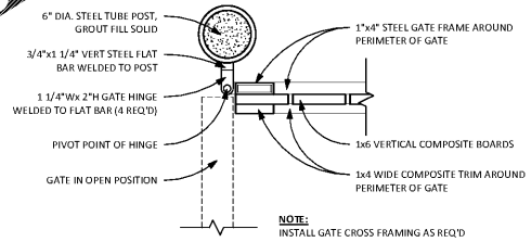
6 TYPICAL HINGE DETAIL A0.3 1 1/2" = 1'-0"
