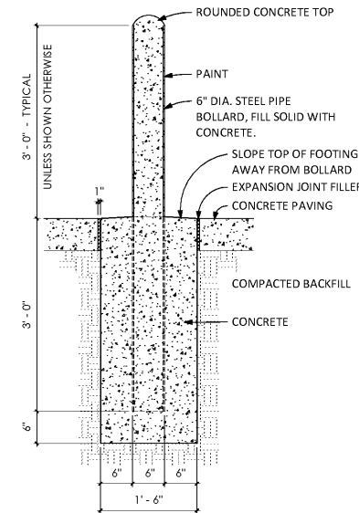
7 TYPICAL BOLLARD DETAIL A0.3 1" = 1'-0"
