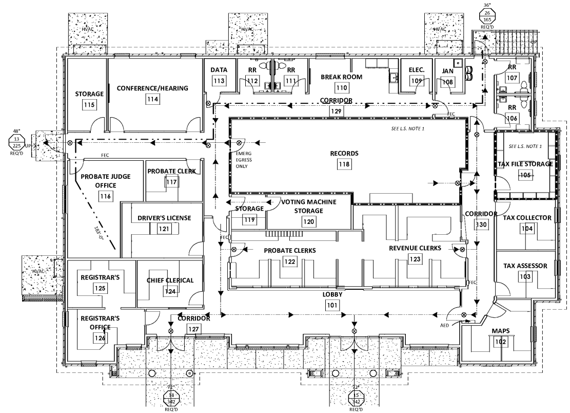
1 LIFE SAFETY PLAN 1/8" = 1'-0"
