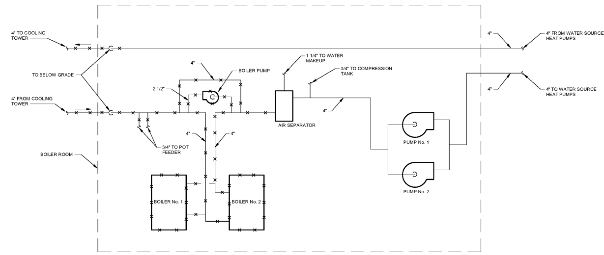
BOILER ROOM PIPING SCHEMATIC - DEMOLITION (ALTERNATE No. 2) NOT TO SCALE
