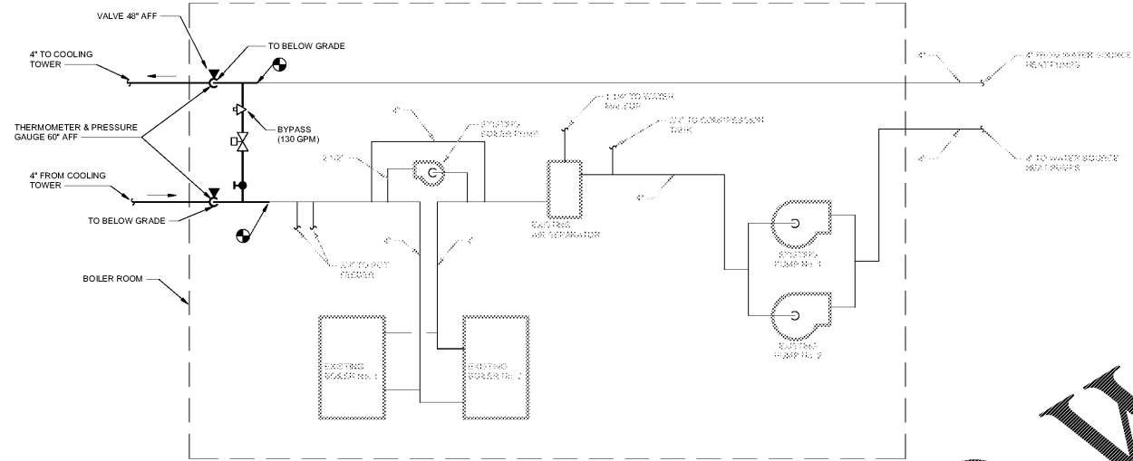
BOILER ROOM PIPING SCHEMATIC - RENOVATION (BASE BID) NOT TO SCALE
