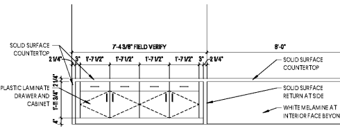
15 ELEVATION - MEDIA DESK SCALE: 3/8"=1'-0"
