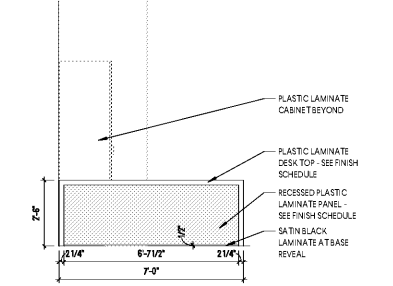
11 ELEVATION - TEACHER DESK SCALE: 3/8"=1'-0"
