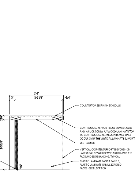
12 MILLWORK SECTION - TEACHER DESK SCALE: 1"=1'-0"
