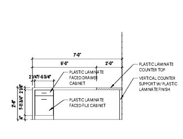
5 ELEVATION - TEACHER DESK SCALE: 3/8"=1'-0"
