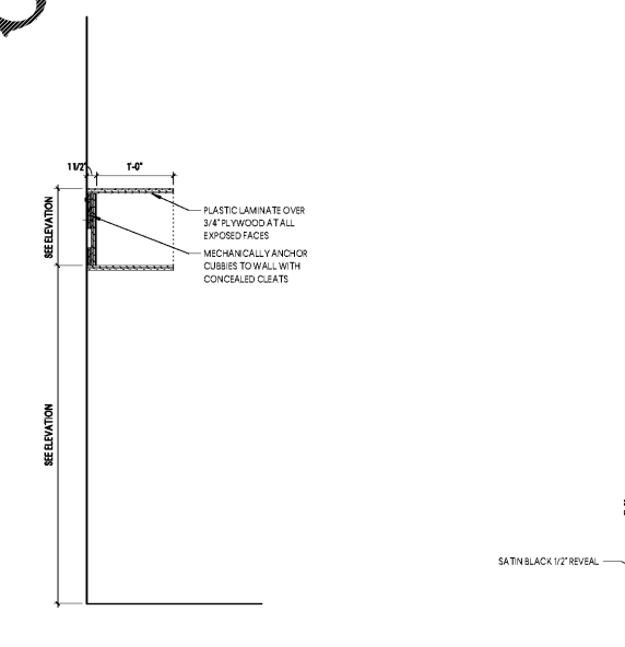
9 MILLWORK SECTION - CUBBIES SCALE: 1"=1'-0"
