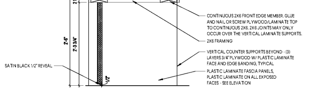
18 MILLWORK SECTION - MEDIA DESK SCALE: 1"=1'-0"
