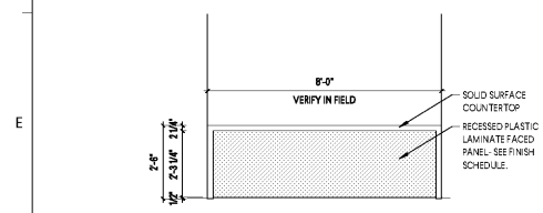
14 ELEVATION - MEDIA DESK SCALE: 3/8"=1'-0"
