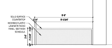
17 ELEVATION - MEDIA DESK SCALE: 3/8"=1'-0"
