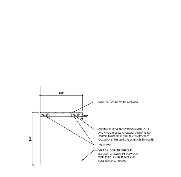
13 MILLWORK SECTION - TEACHER DESK (wall) SCALE: 1"=1'-0"
