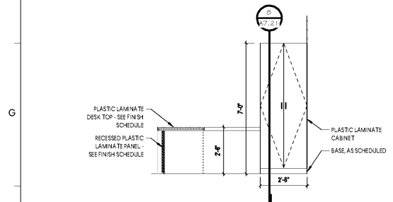
6 ELEVATION - TEACHER DESK SCALE: 3/8"=1'-0"
