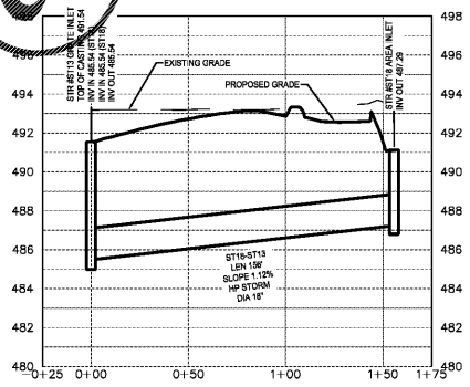
ST18-ST13 Horizontal Scale: 1" = 40' Vertical Scale: 1" = 4'
