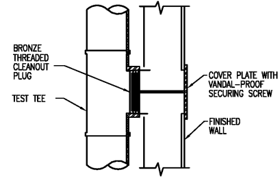
1 WALL CLEAN OUT DETAIL P-6 NOT TO SCALE
