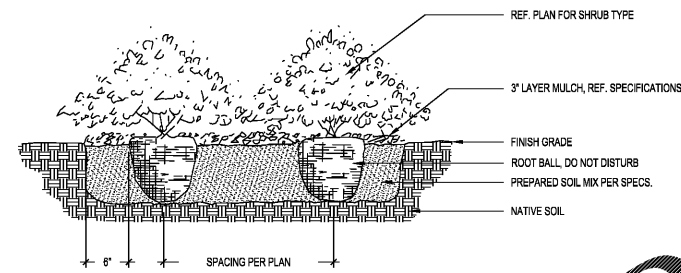
B SHRUB PLANTING SECTION TO SCALE
