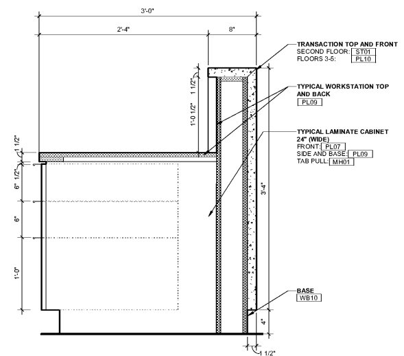
3 NURSE STATION - SECTION THROUGH COUNTER 1/12" = 1'-0"
