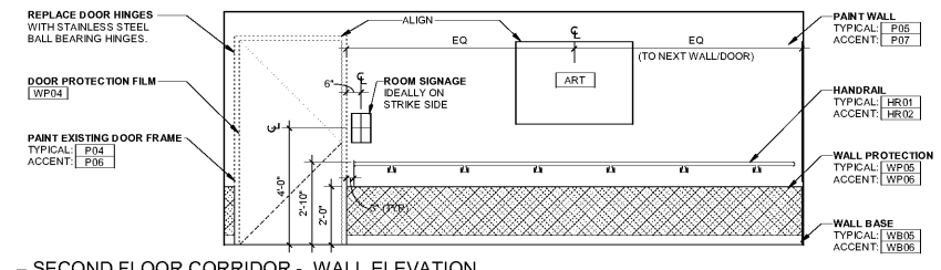
5 SECOND FLOOR CORRIDOR - WALL ELEVATION 3/8" = 1'-0"
