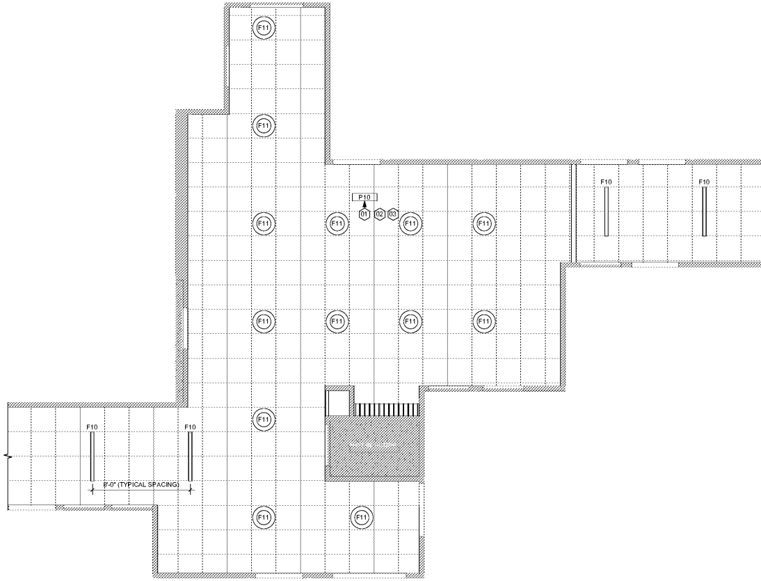
4 SHORT TERM CORRIDOR - RCP 1/4" = 1'-0"
