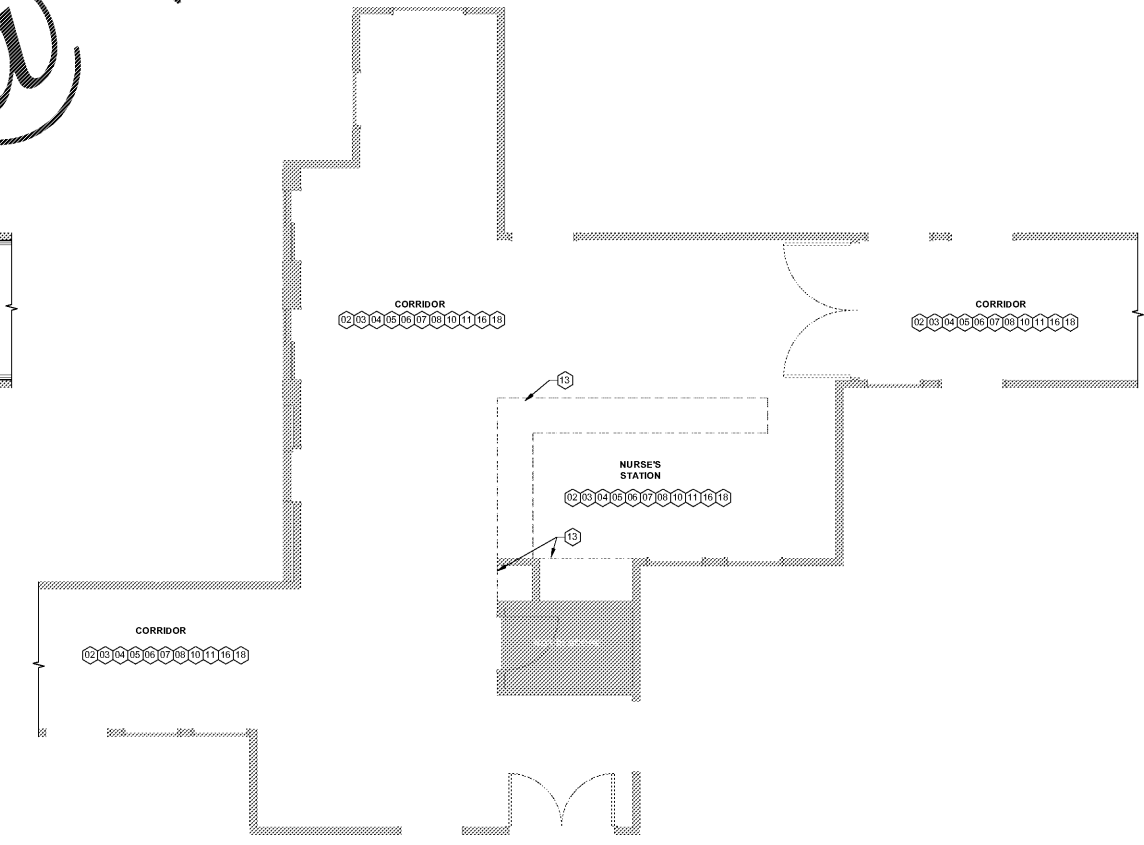
1 2ND FLOOR NURSE STATION AND CORRIDOR - DEMOLITION PLAN 1/4" = 1'-0"
