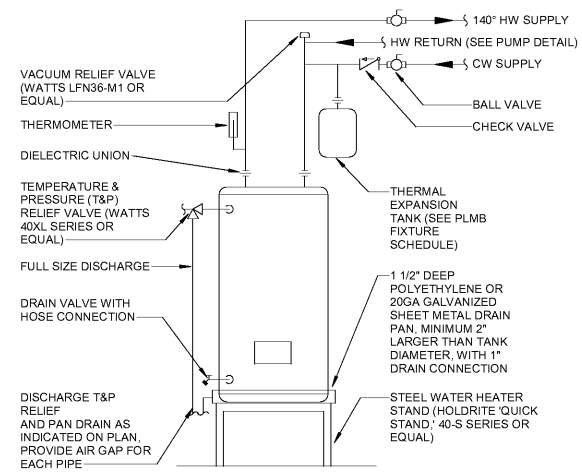
1 STAND MOUNTED ELECTRIC WATER HEATER P0.3 N.T.S.
