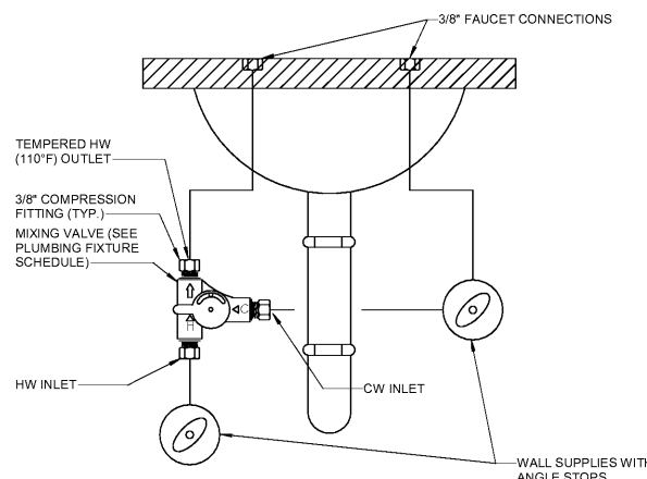
8 POINT OF USE MIXING VALVE (MV-2) P0.3 N.T.S.
