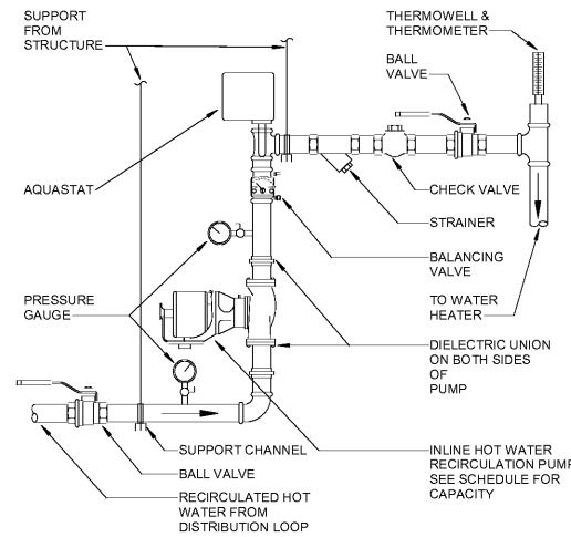
2 HOT WATER RECIRCULATION PUMP P0.3 N.T.S.
