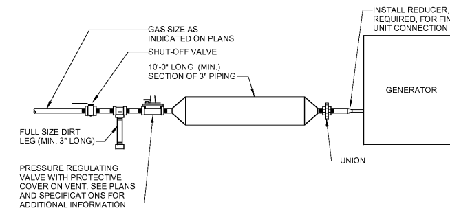
9 EQUIPMENT GAS CONNECTION P0.3 N.T.S.
