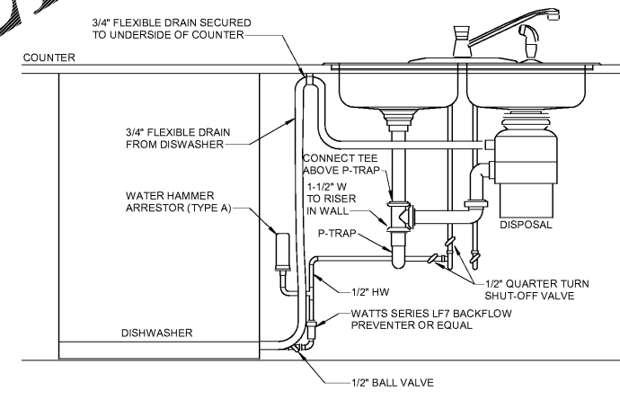
6 DISHWASHER CONNECTION P0.3 N.T.S.
