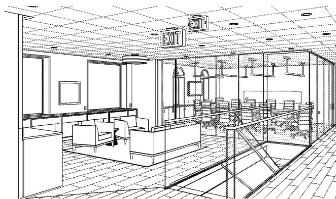
5 2ND FLOOR STAIR & CONF/LOBBY ID-5.5
