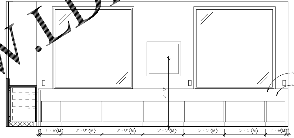
3 201 UPPER LOBBY/ LIBRARY- SOUTH ID-2.5 1/2" = 1'-0"
