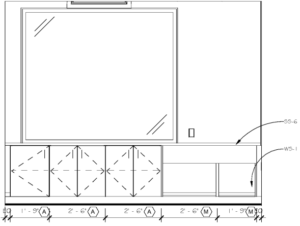
2 203 OFFICE 2- SOUTH ID-2.5 1/2" = 1'-0"
