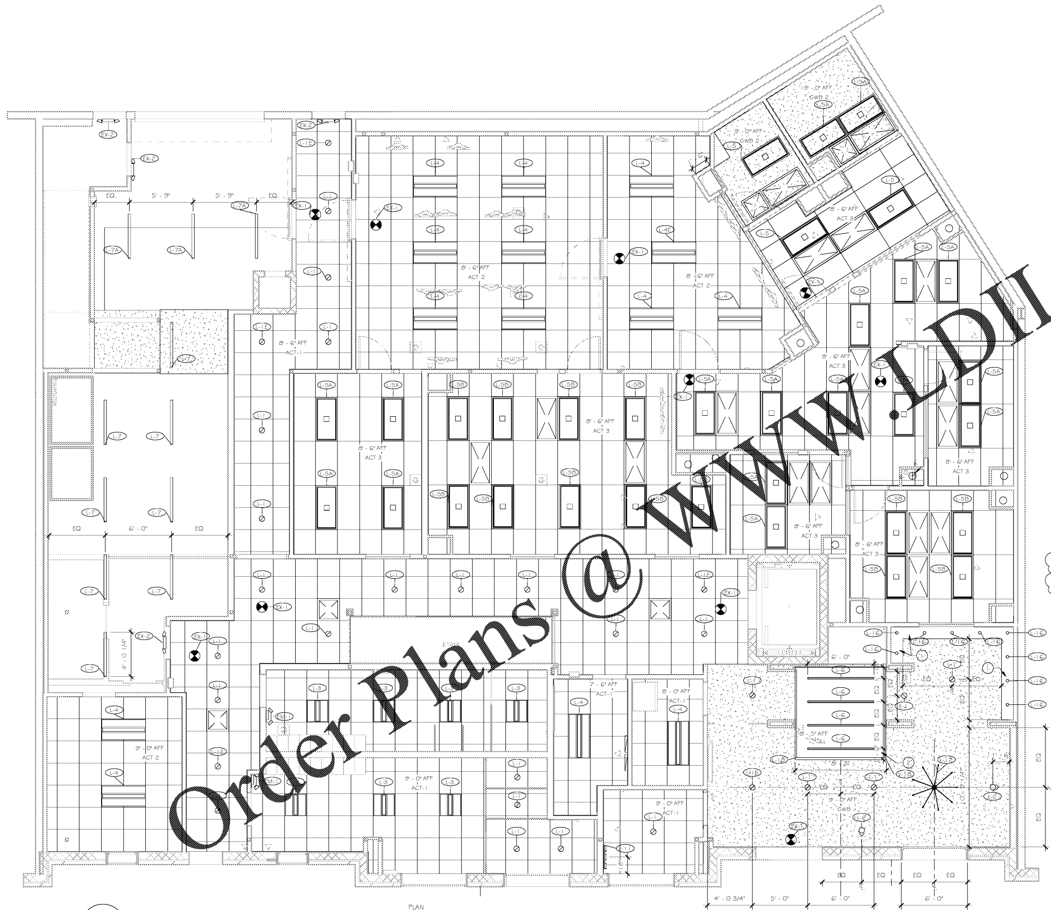
REFLECTED CLG. PLAN - 1ST FLR. A-2.1 1/4" = 1'-0" PLAN NORTH
