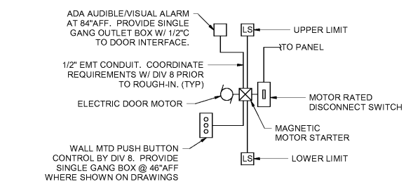
5 SCHEMATIC - COIL DOOR CONNECTION NO SCALE
