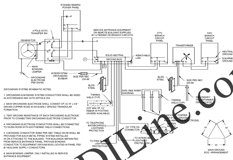
4 SCHEMATIC - 480V ELECTRICAL GROUNDING SYSTEM NO SCALE
