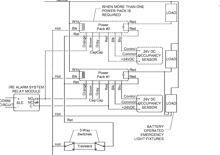
6 SCHEMATIC - CONNECTION OF LIGHT FIXTURES & OCCUPANCY SENSORS IN CORRIDORS, PASSAGeways, HALLWAYS, LOBBIES, AND COMMONS NO SCALE
