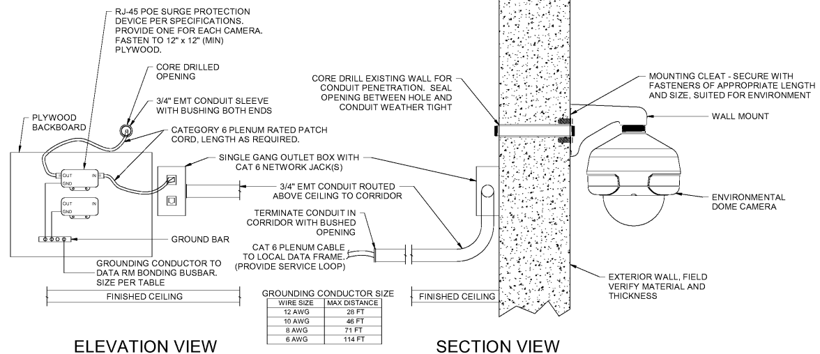
2 DETAIL - INSTALLATION OF IP CAMERA DATA DROP FOR EXTERIOR CAMERAS NO SCALE
