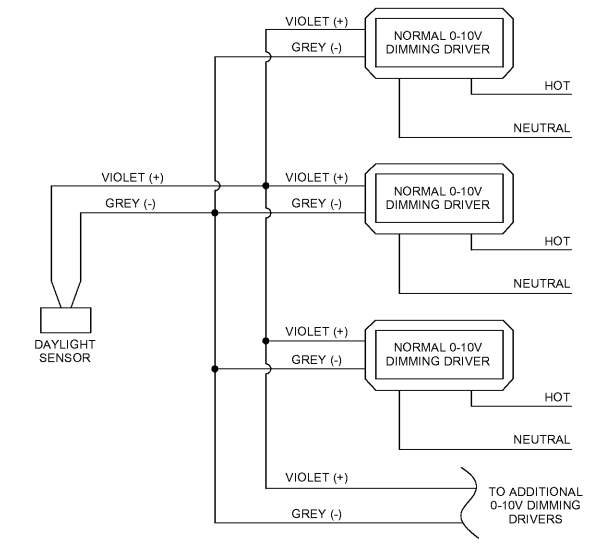
8 SCHEMATIC - DAYLIGHT SENSOR DIMMING CONTROL NO SCALE
