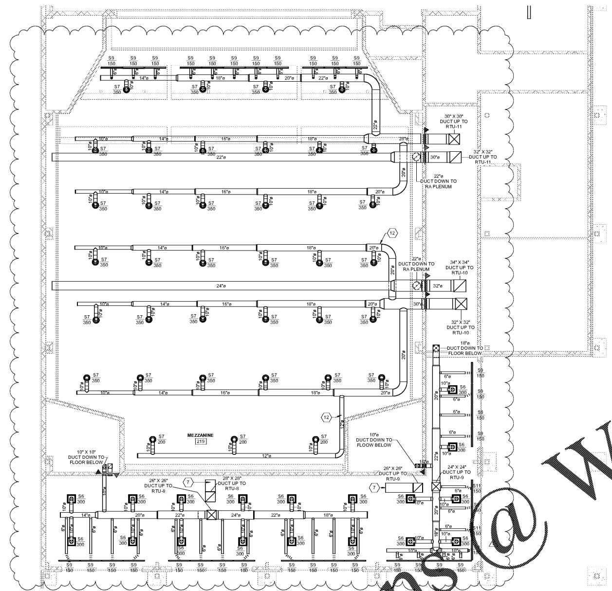
1 LEVEL 02 MECHANICAL PLAN - AUD - LOBBY 1/8" = 1'-0"
