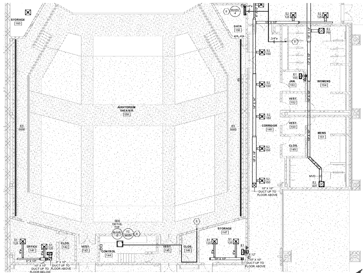
1 LEVEL 01 MECHANICAL PLAN - AUDITORIUM 1/8" = 1'-0"
