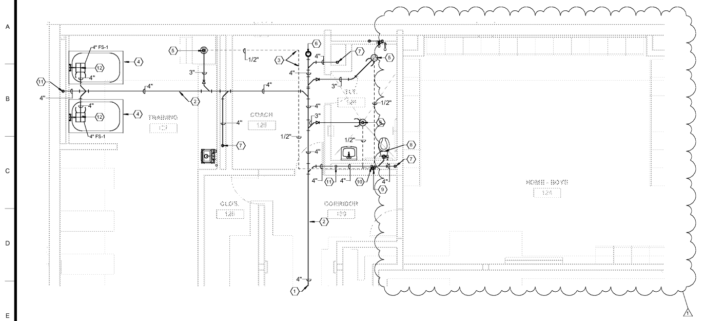
1 ENLARGED PLUMBING BELOW FLOOR PLAN HOME - BOYS 124 - LEVEL 1 1/4\" = 1'-0"
