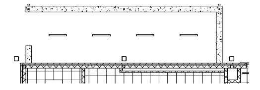
2 RCP - LEVEL 02 - GYMNASIUM - EXTERIOR COOKING AREA 1/8" = 1'-0"
