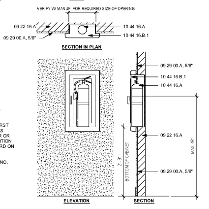
2 SEMI-RECESSED FIRE EXTINGUISHER @ GYP. BD. & MTL STUD 3/4" = 1'-0"
