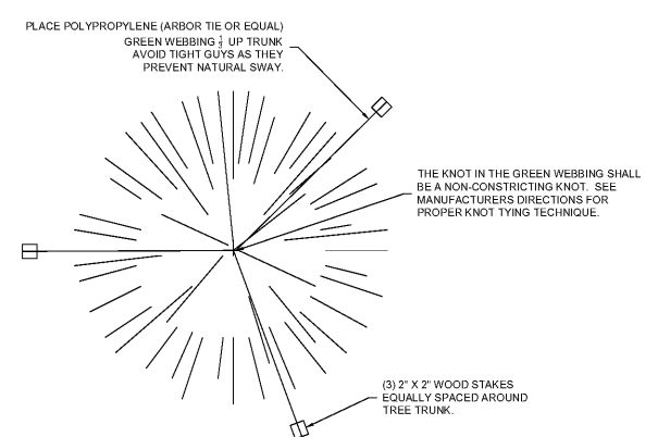
TYPICAL TREE STAKING DETAIL NOT TO SCALE
