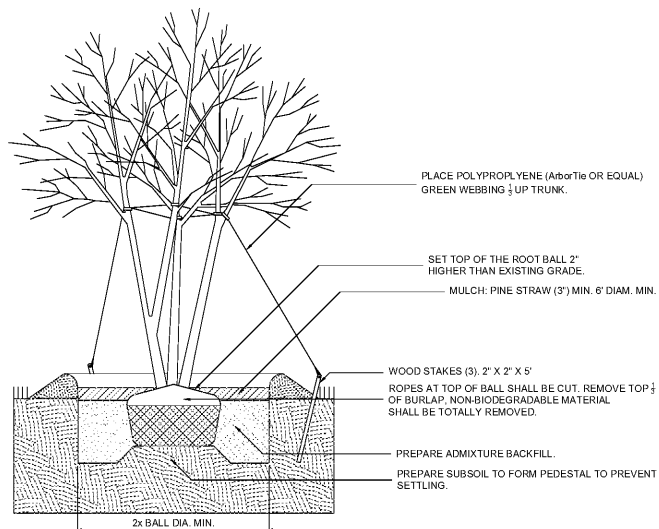
MULT-STEM TREE INSTALLATION DETAIL NOT TO SCALE
