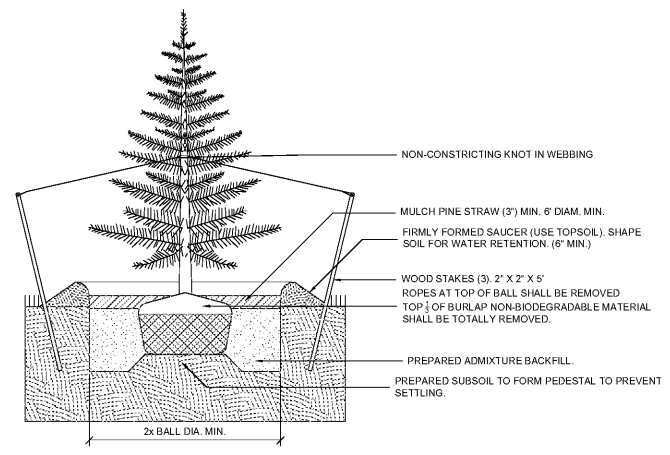
EVERGREEN TREE INSTALLATION DETAIL NOT TO SCALE
