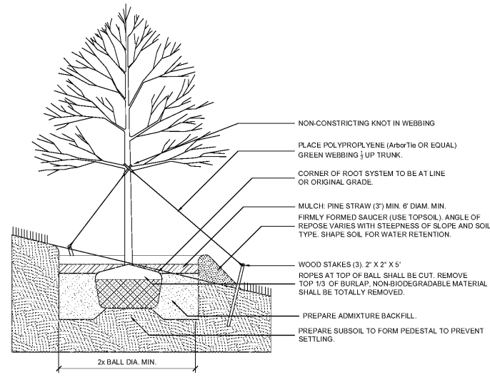
TREE INSTALLATION ON SLOPES DETAIL NOT TO SCALE UP TO 4:1 SLOPES
