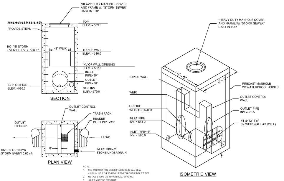
OUTLET STRUCTURE DETAIL NOT TO SCALE
