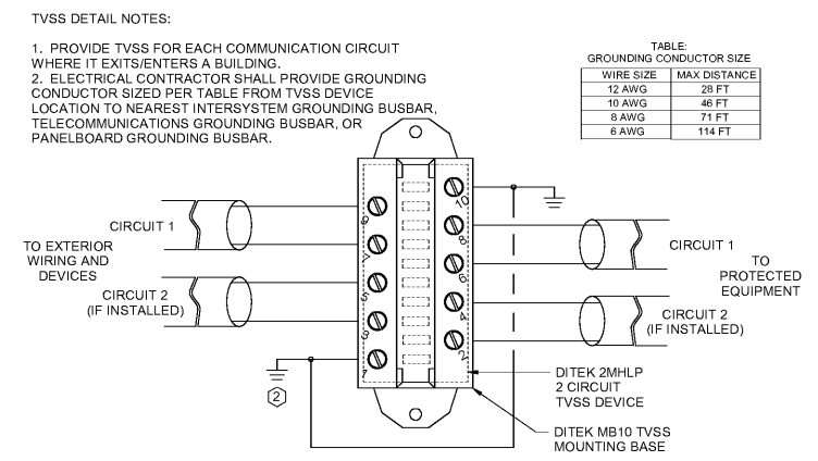
3 DETAIL - TRANSIENT VOLTAGE SURGE SUPPRESSION (TVSS) NO SCALE
