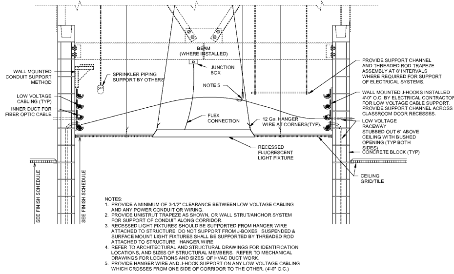
1 DETAIL - SUPPORT OF ELECTRICAL APPARATUS IN CORRIDORS NO SCALE
