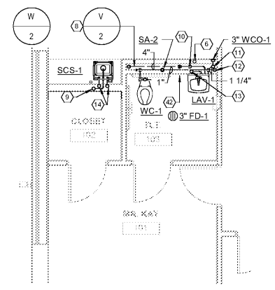
2 ENLARGED PLUMBING ABOVE FLOOR PLAN - TOILET #2 - LOWER LEVEL 1/4" = 1'-0"
