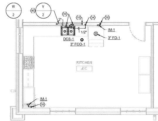
4 ENLARGED PLUMBING ABOVE FLOOR PLAN - KITCHEN - UPPER LEVEL 1/4" = 1'-0"
