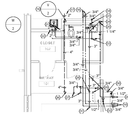
3 ENLARGED PLUMBING ABOVE CEILING PLAN - TOILET #2 - LOWER LEVEL 1/4" = 1'-0"
