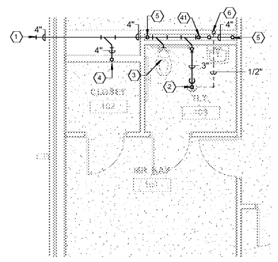
1 ENLARGED PLUMBING BELOW FLOOR PLAN - TOILET #2 - LOWER LEVEL 1/4" = 1'-0"
