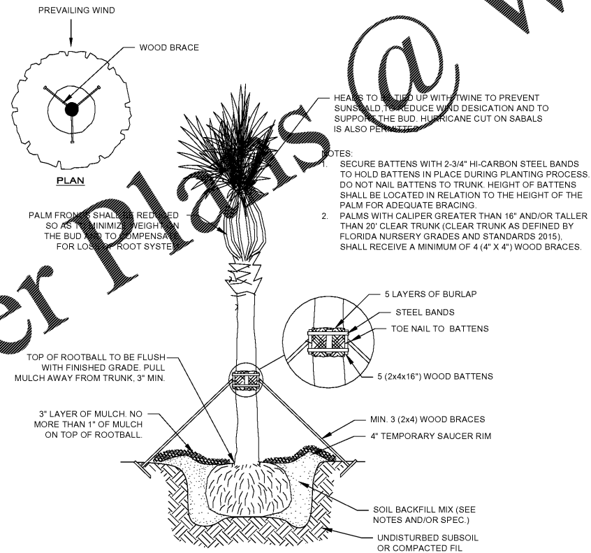
TYPICAL SINGLE TRUNK PALM N.T.S.
