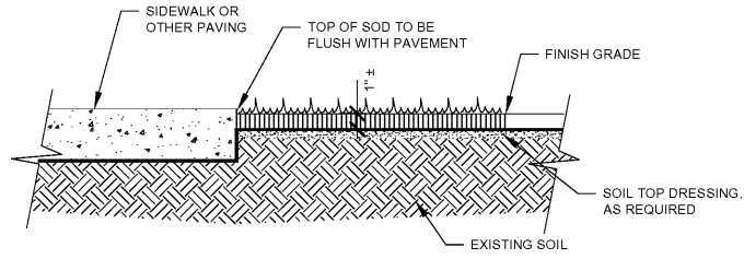
TYPICAL SOD PLANTING N.T.S.
