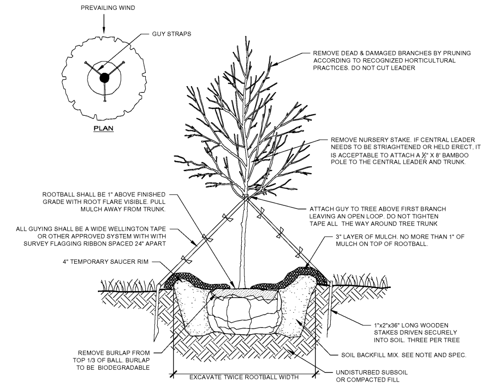
TYPICAL TREE INSTALLATION N.T.S.
