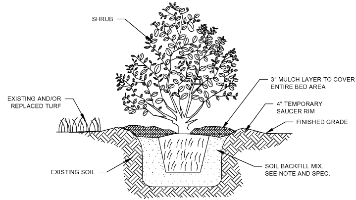
TYPICAL SHRUB PLANTING N.T.S.
