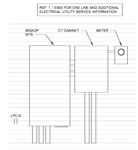
8 ELECTRICAL SERVICE 1/2" = 1'-0"
