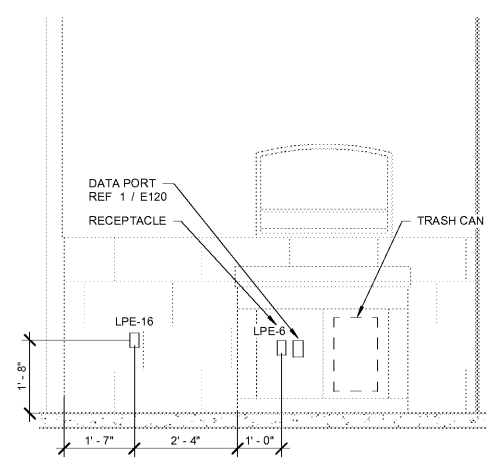
2 LOTTERY STATION ELEVATION 1/2" = 1'-0"
