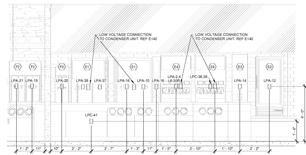
1 CHILL ZONE ELEVATION 1/2" = 1'-0"
