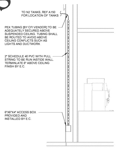
7 N2 TANK LINE CONDUIT ROUTING 1/2" = 1'-0"
