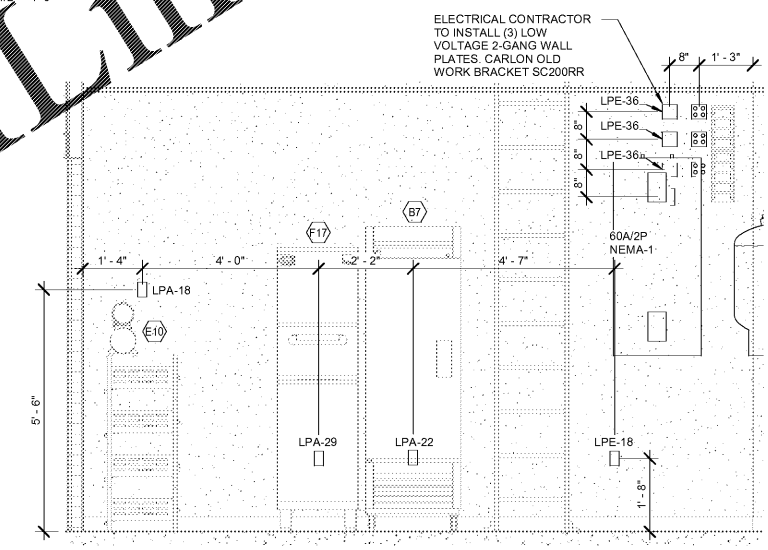
3 COFFEE BAR ELEVATION 1/2" = 1'-0"
