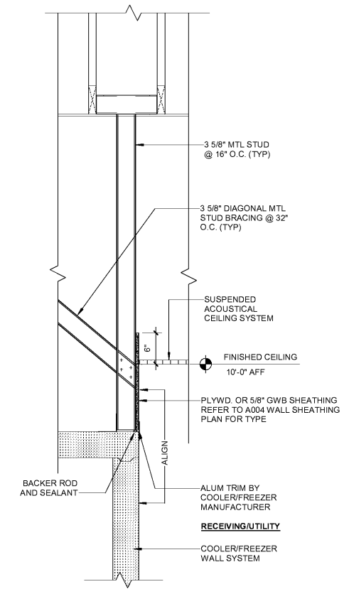
1 SOFFIT @ COOLER/FREEZER (RECEIVING) 1" = 1'-0"
