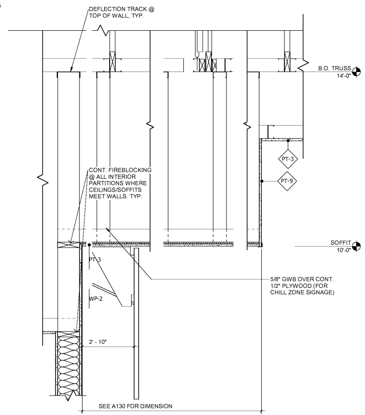
2 SOFFIT @ CHILLZONE 1" = 1'-0"
