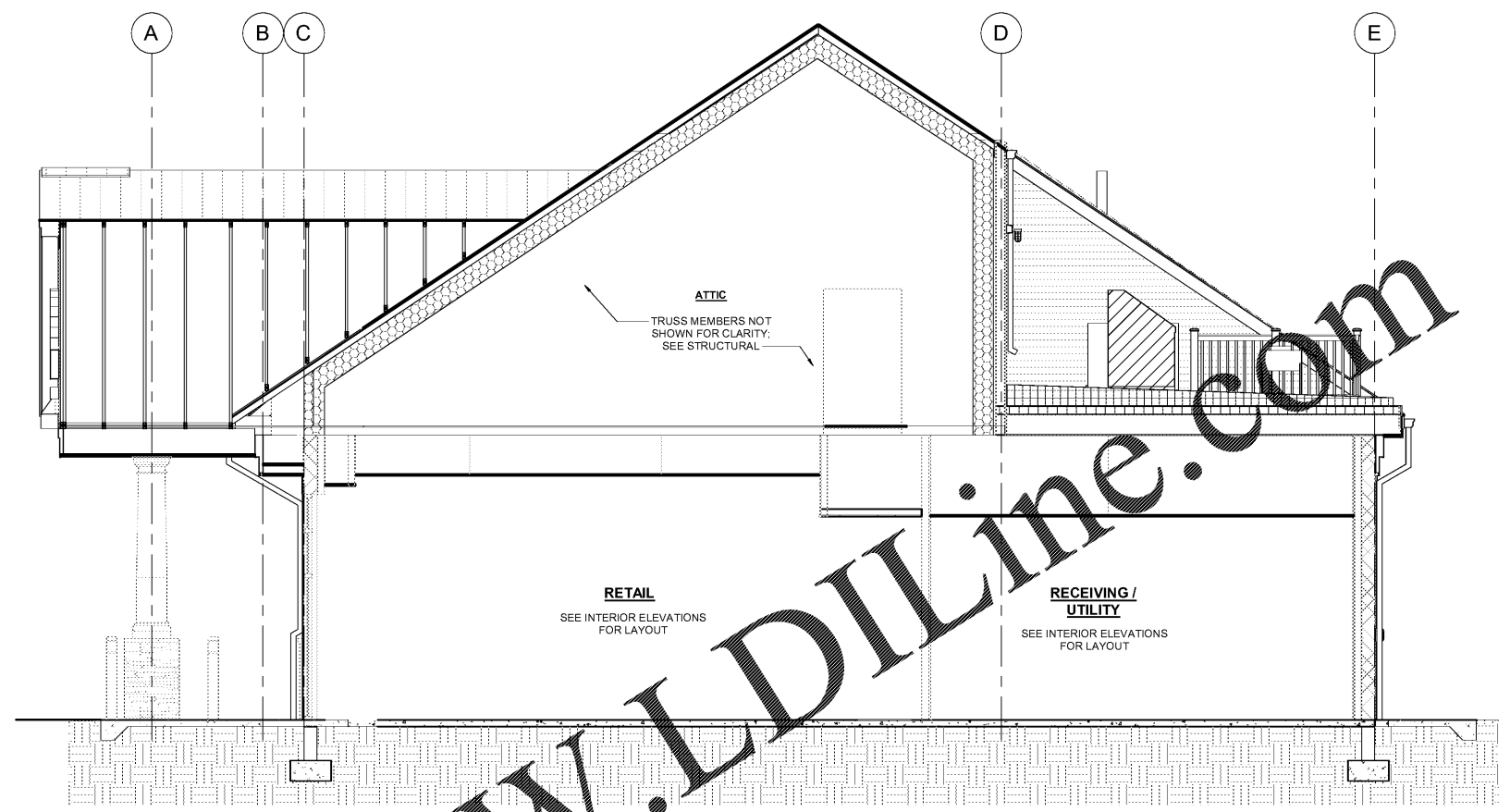
② CROSS SECTION @ CANOPY/FLAT ROOF 1/4" = 1'-0"
