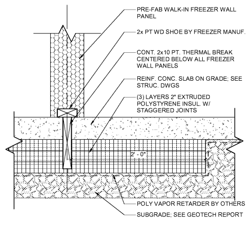
② THERMAL BREAK @ FREEZER WALL/DOOR 1 1/2" = 1'-0"
