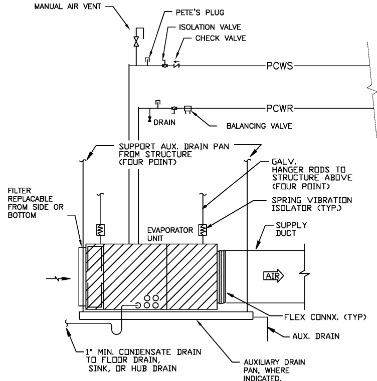
1 FAN COIL COOLING UNIT M401 NO SCALE
