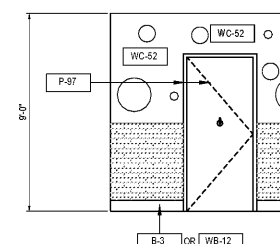
RESTROOM ELEVATION
