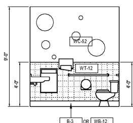
RESTROOM ELEVATION
