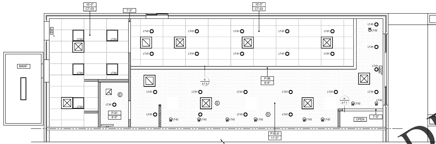
REFLECTED CEILING PLAN (A)
