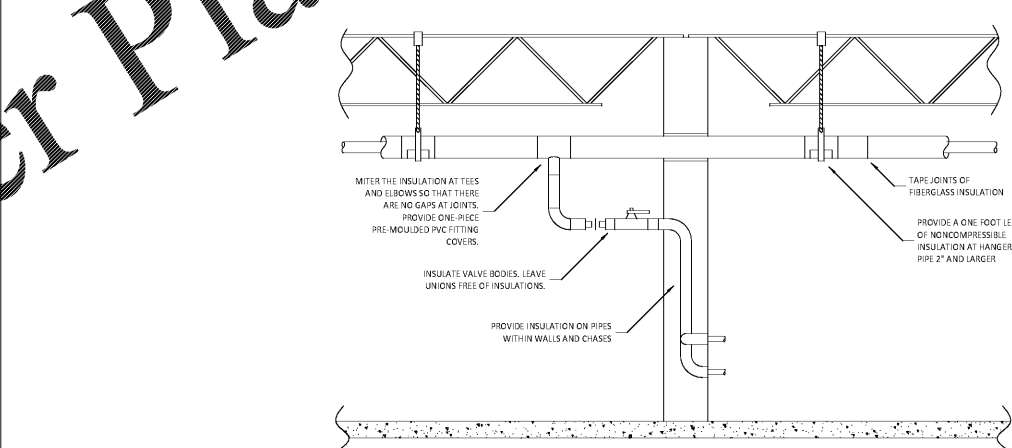
2 PIPE INSULATION DETAIL NOT TO SCALE
