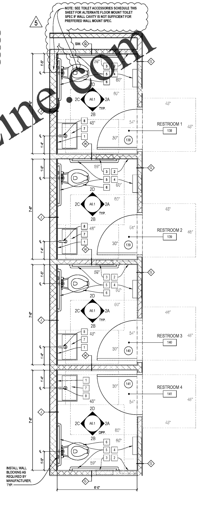
A RESTROOM DIMENSION PLAN SCALE: 1/4" = 1'-0"
