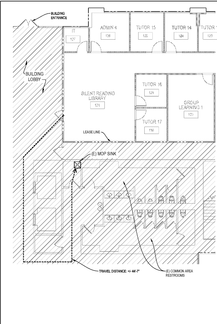
3 PATH OF TRAVEL TO COMMON AREA MOP SINK SCALE: N.T.S.
