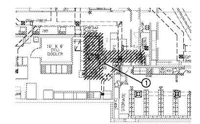
5B HVAC DEMO PLAN - MAIN LEVEL SCALE: 1/8" = 1'-0"
